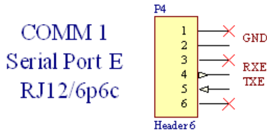
FIG. 9 NeXGen™ CCURX Local Port Pin-Out (for PCB revision A through D)
