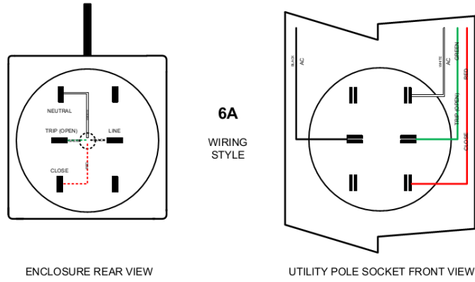
FIG. 5 NeXGen™ CCURX 6A Wiring Diagram
