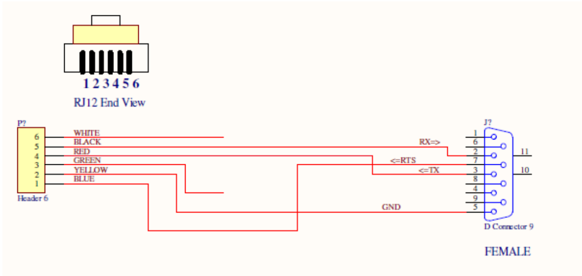
FIG. 8 NeXGen™ TAC-01 Series Local Cable
