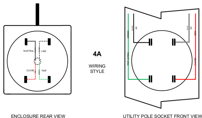
FIG. 4 NeXGen™ CCURX 4A Wiring Diagram
