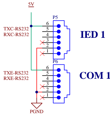
FIG. 10 NeXGen™ CCURX IED Port 1 Pin-Out
