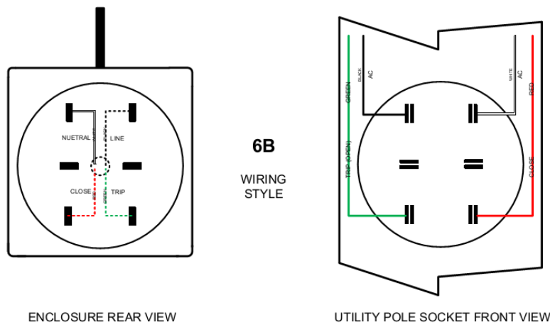
FIG. 6 NeXGen™ CCURX 6B Wiring Diagram
